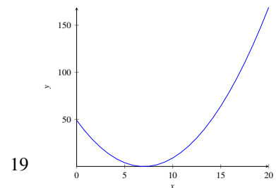
Figure 1.9: Plot of (x - 7)^2
